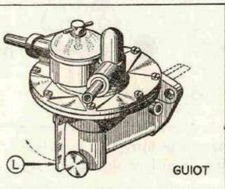
Fig. 3. — POMPES A ESSENCE.
