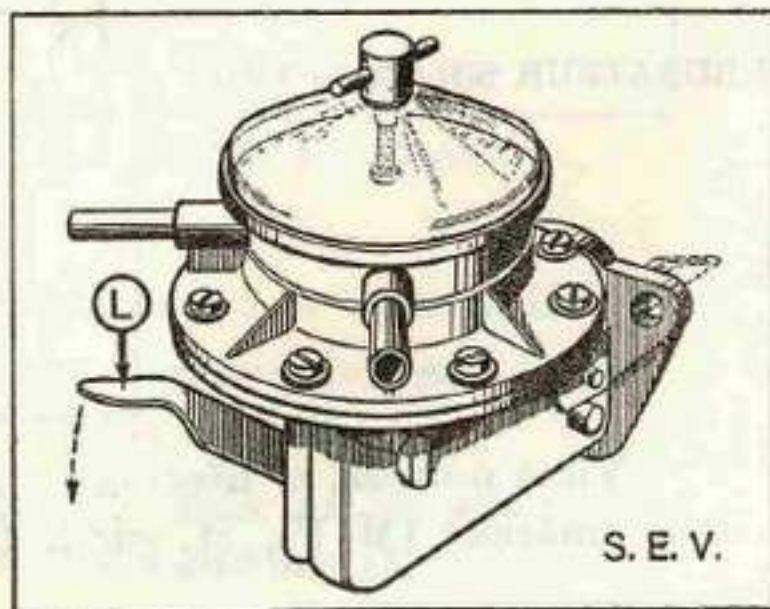
Fig. 3. — POMPES A ESSENCE.
